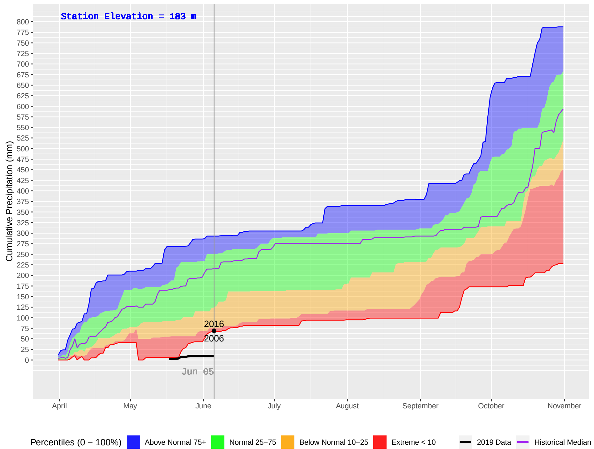
MESACHIE 2 (934) : Historical (2006–2018), Current (2019) Daily Cumulative Precipitation
