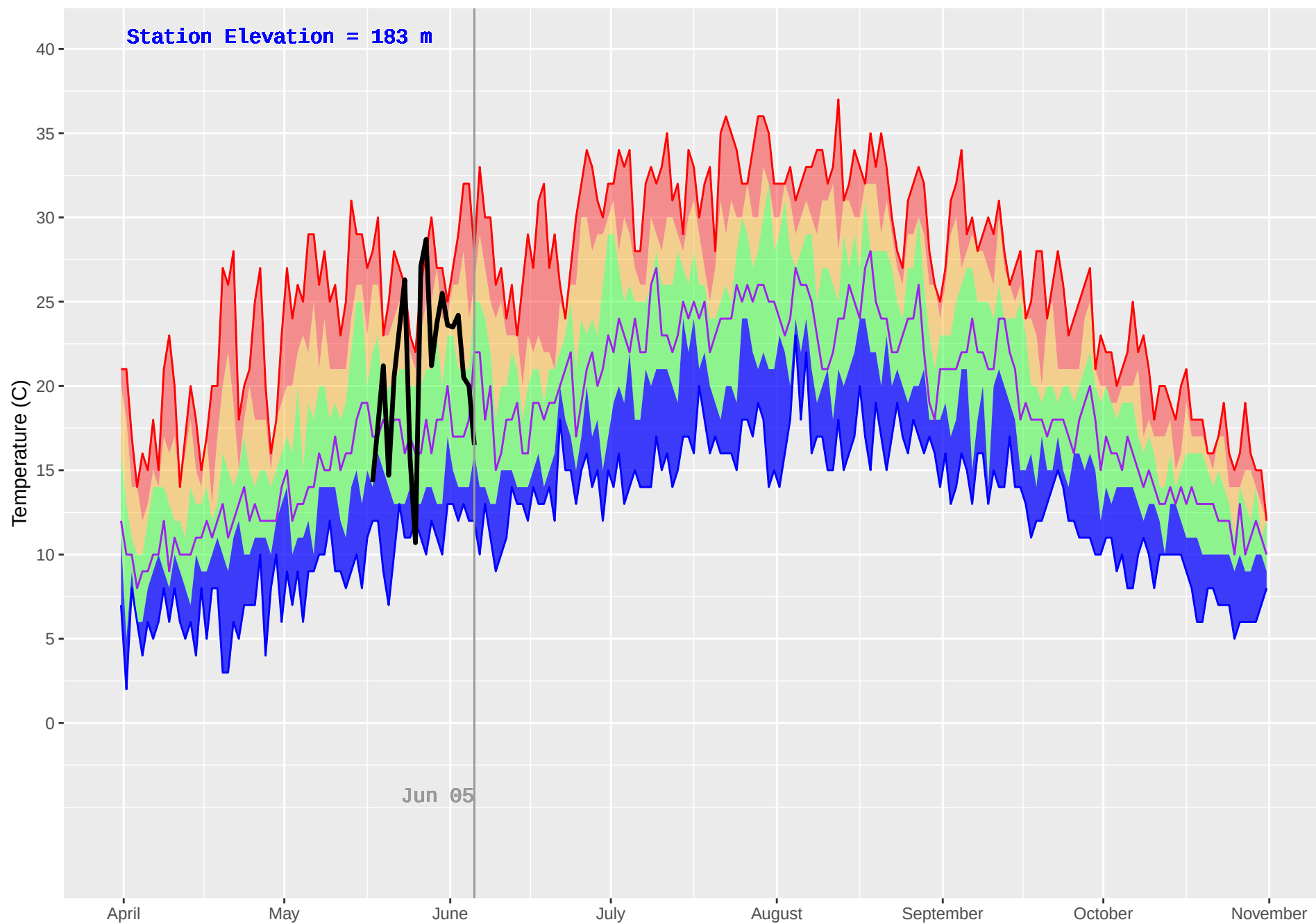
MESACHIE 2 (934) : Historical (2006–2018) and Current (2019) Daily Temperature
