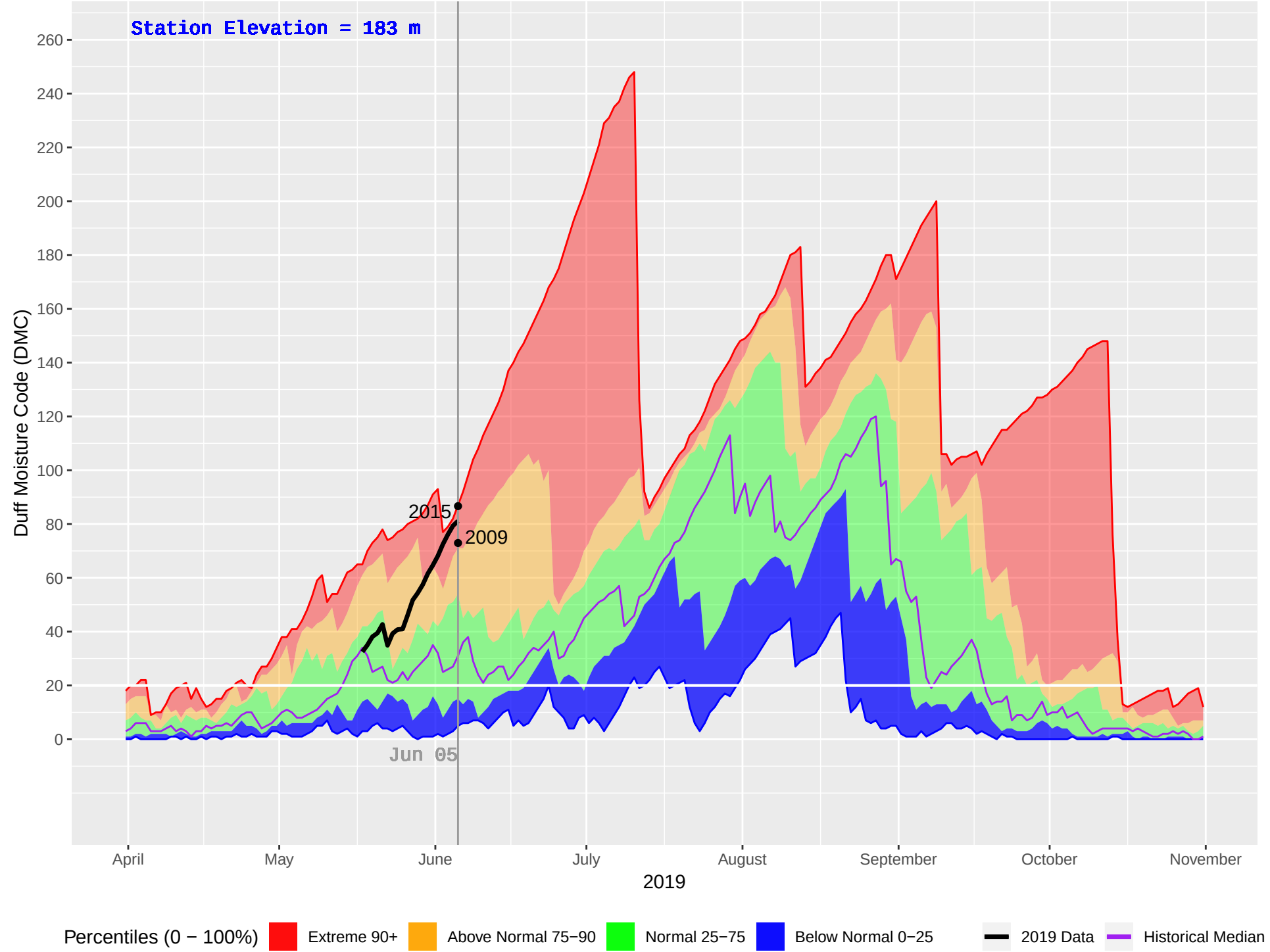
MESACHIE 2 (934) : Historical (2006–2018), Current (2019) Daily Duff Moisture Code (DMC)
