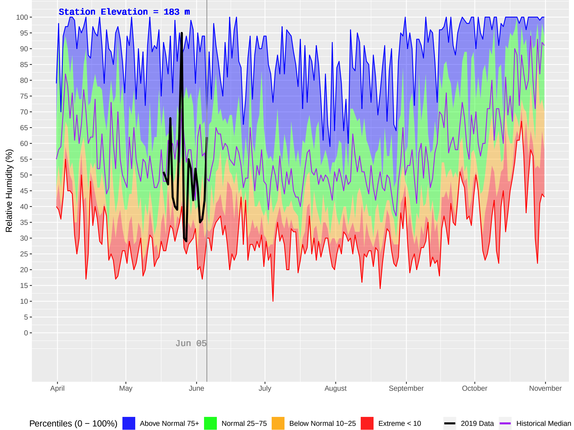
MESACHIE 2 (934) : Historical (2006–2018) and Current (2019) Daily Relative Humidity
