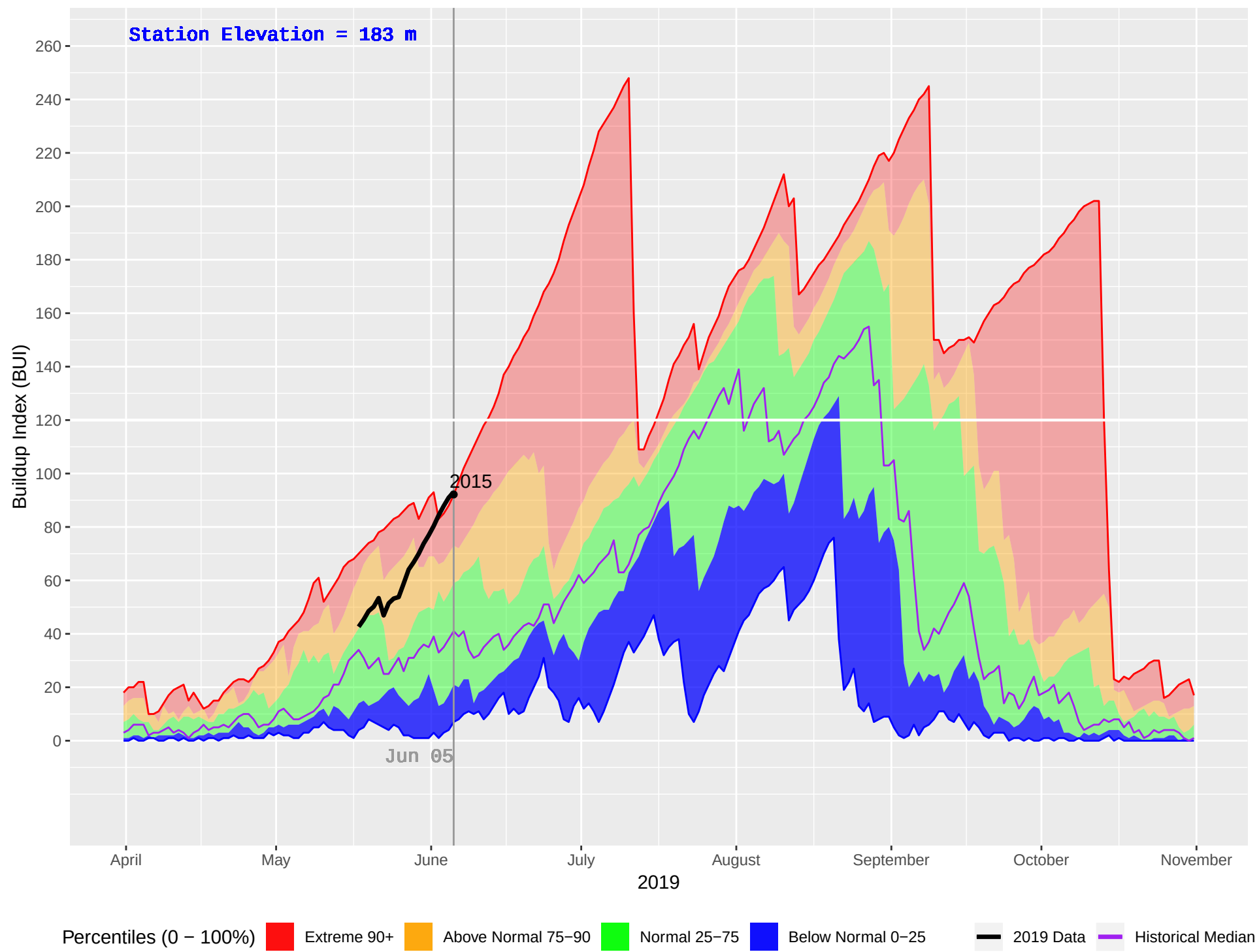
MESACHIE 2 (934) : Historical (2006–2018), Current (2019) Daily Buildup Index (BUI)
