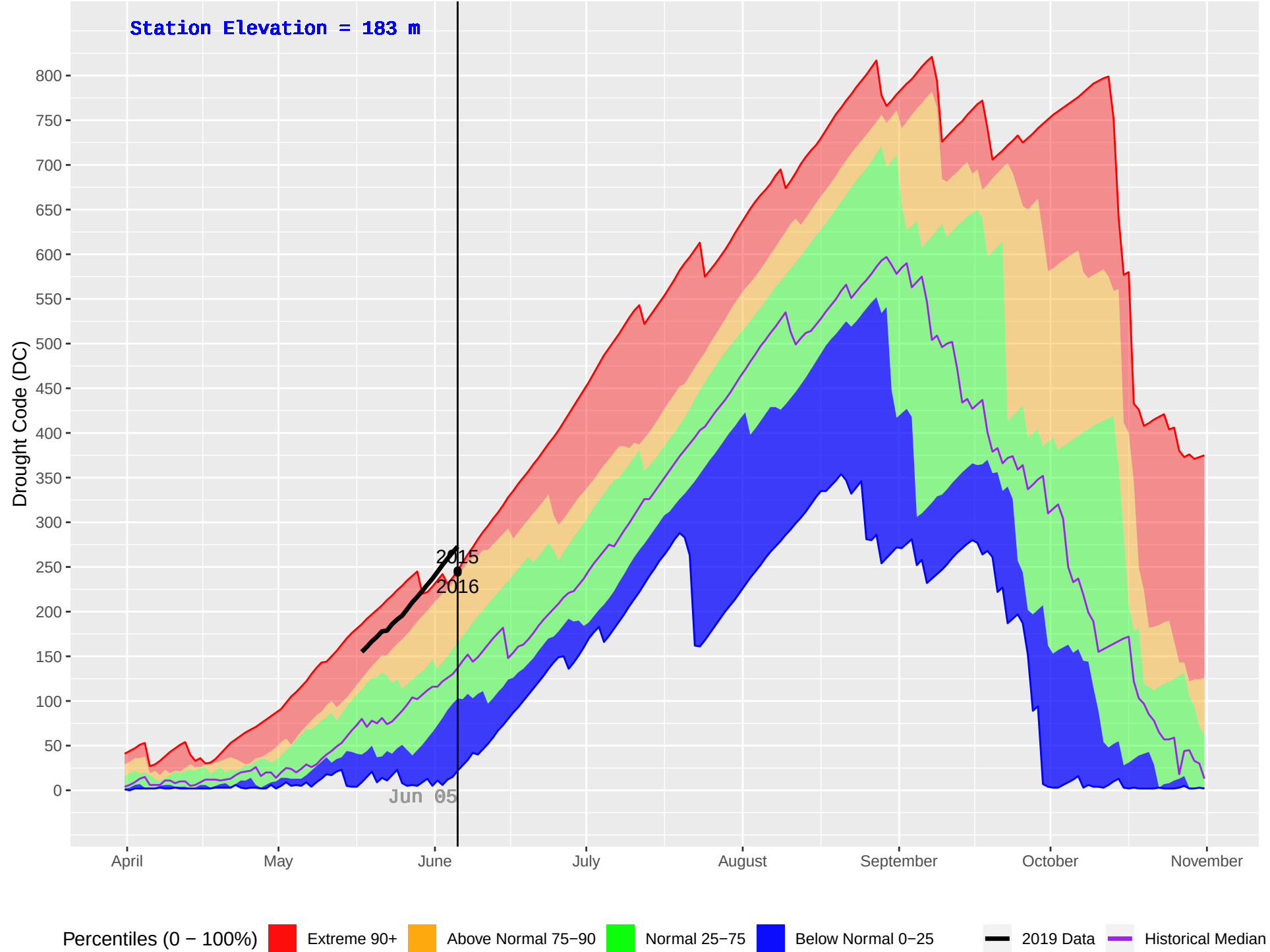
MESACHIE 2 (934) : Historical (2006–2018) and Current (2019) Daily Drought Code (DC)
