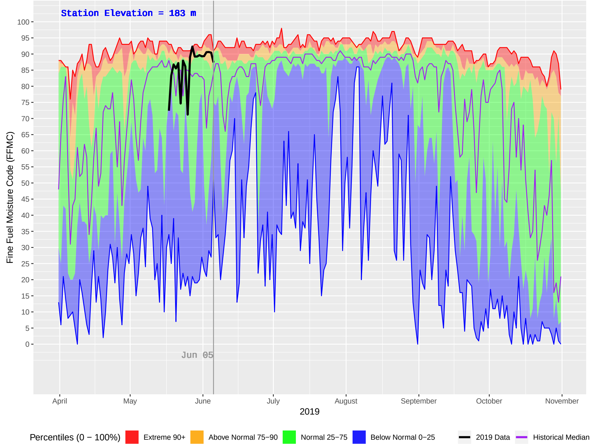
MESACHIE 2 (934) : Historical (2006–2018) and Current (2019) Daily Fine Fuel Moisture Code (FFMC)
